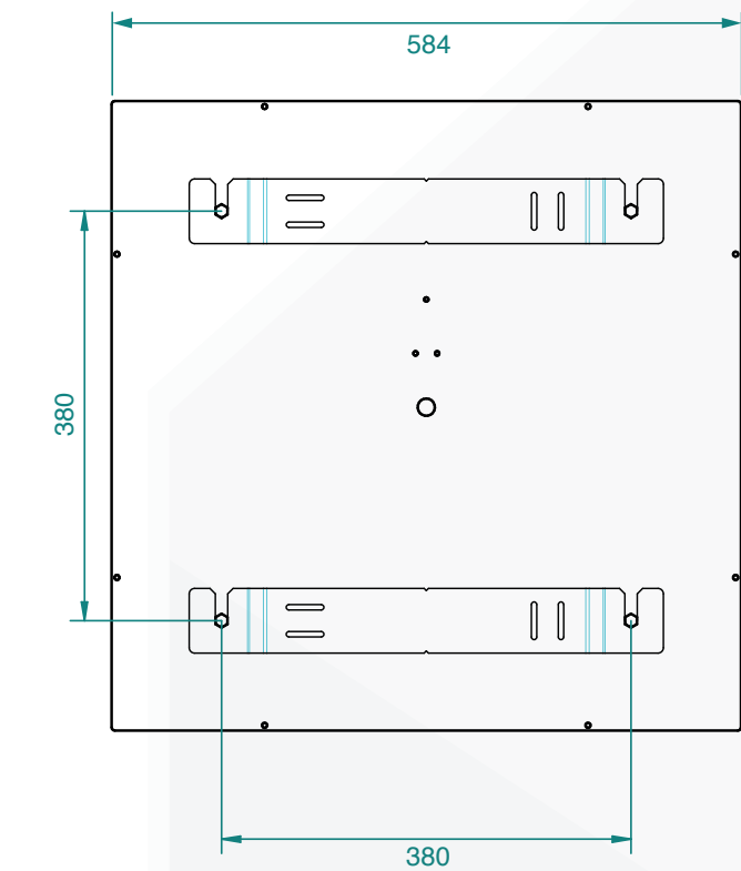
Backside Leranti® Easy/HTP 60x60
