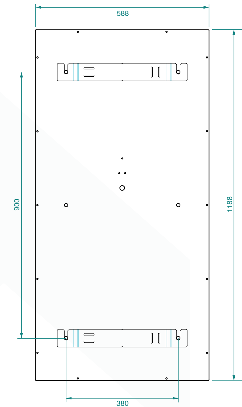
Backside Leranti® Easy/HTP 60x120
