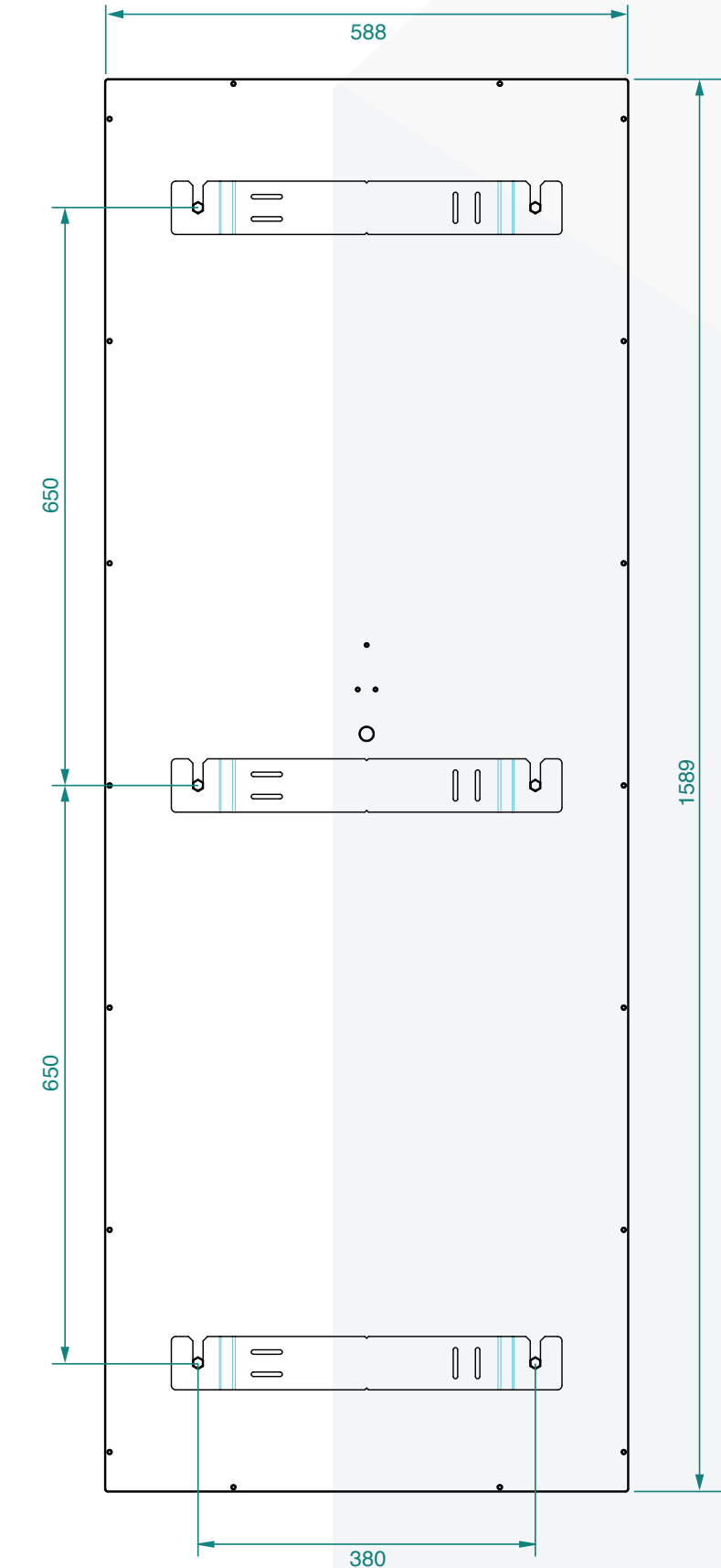
Backside Leranti® Easy/HTP 60x160
